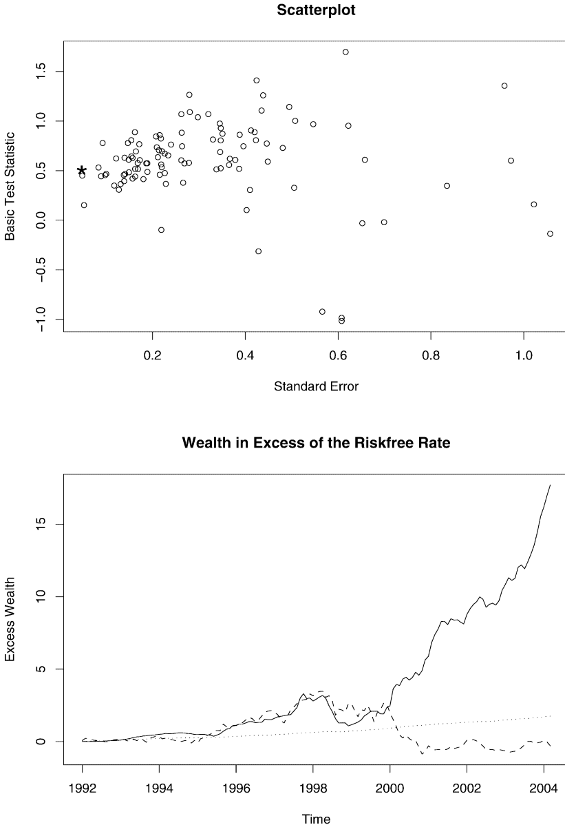
FIGURE 1.—Top: Scatterplot of the basic test statistics w_{147,s} against the standard errors \hat{\sigma}_{147,s} in the empirical application of Section 9. The point (0.0476, 0.5062) , which corresponds to the largest studentized statistic z_{147,s} = w_{147,s}/\hat{\sigma}_{147,s} , is marked by the symbol *. Bottom: The cumulative wealth in excess of the risk-free rate, given an initial investment of 1, over the investment period 01/1992 until 03/2004 for three hedge funds: the one with the largest basic test statistic w_{147,s} (solid line), the one with the largest studentized statistic z_{147,s} (dotted line), and the one with the largest standard error \hat{\sigma}_{147,s} (dashed line).
